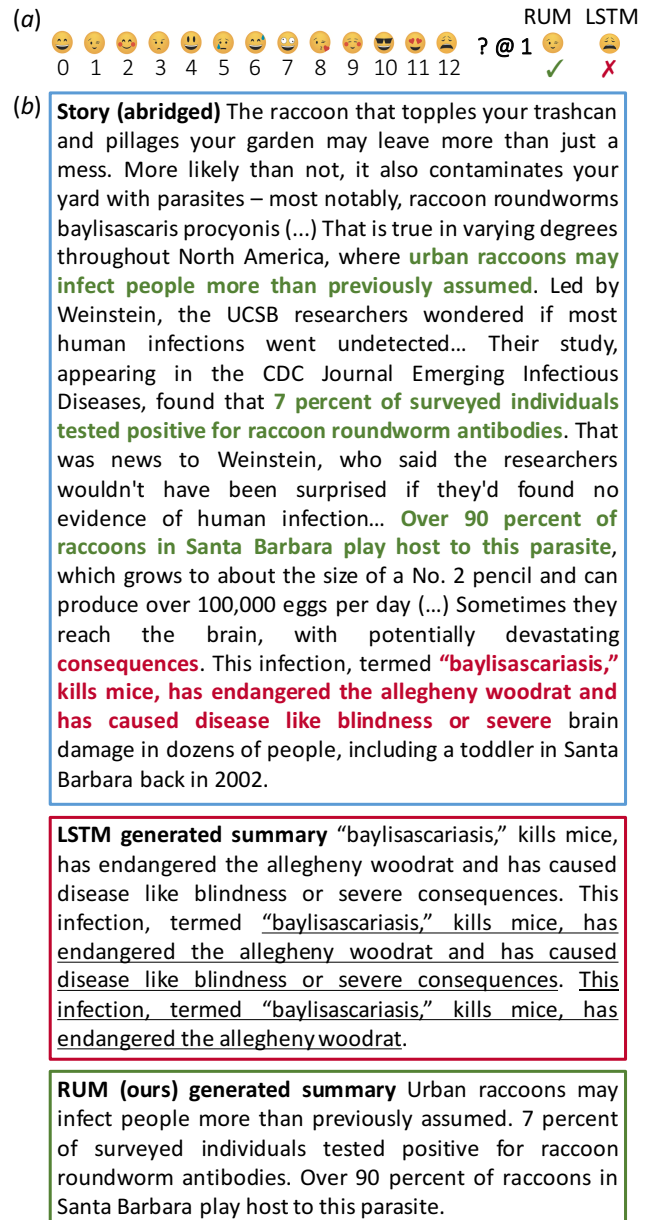
Figure 1: RUM vs. LSTM (a) Synthetic sequence of emojis: a RUM-based RNN recalls the emoji at position 1 while LSTM does not. (b) Text summarization: a seq2seq model with RUM recalls relevant information while LSTM generates repetitions near the end.
